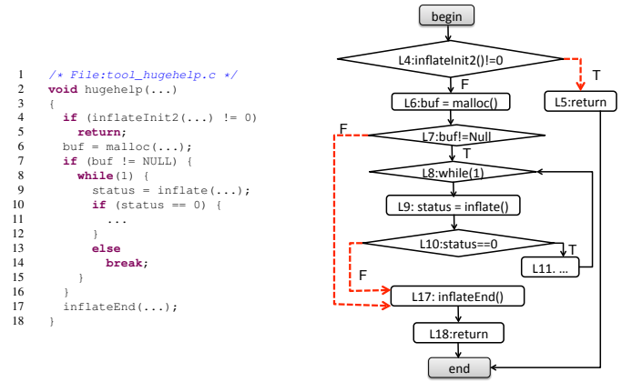
Figure 1: Sample error handling code and the corresponding Control Flow Graph (CFG) containing zlib and libc API functions adapted from Curl. The red, dotted arrows show error branches.
