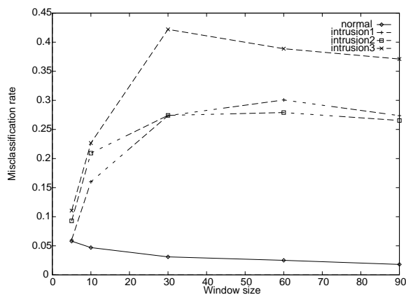
Figure 1: Effects of Window Sizes on Misclassification Rates
